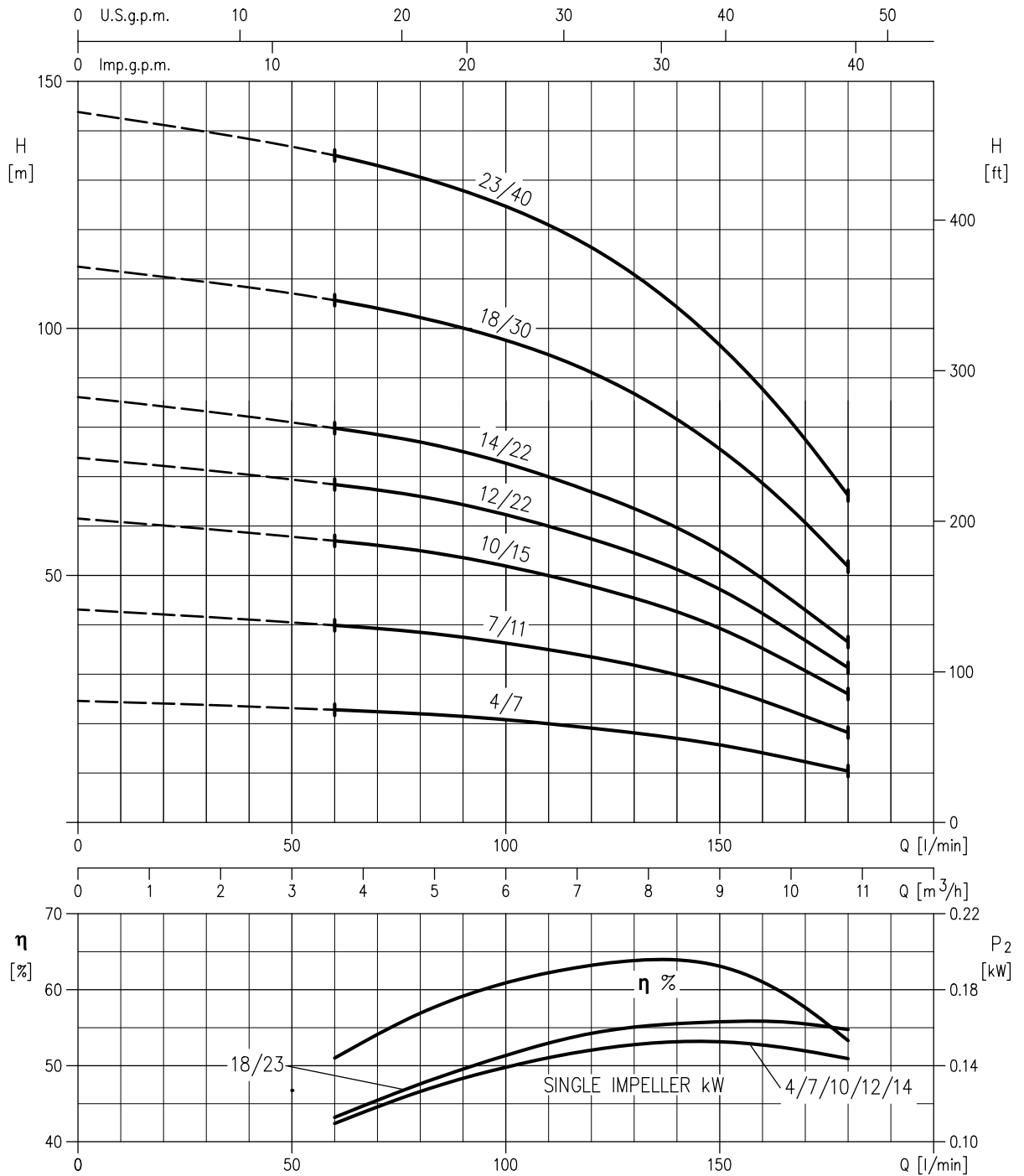
4BHS7 - MEI > 0.40- Impeller diameter = 74 mm
